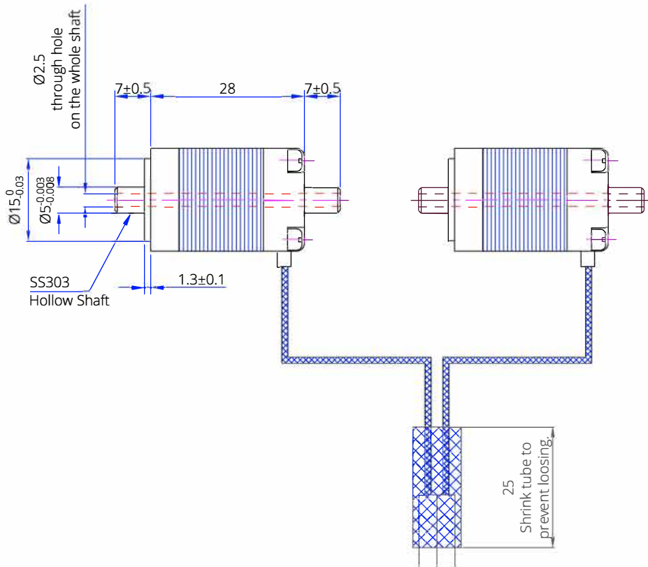
2 motors connector to one Dupon Connector 2X4Pin 2.54mm
